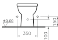
With side holes
