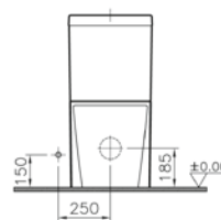
Concealed cistern
