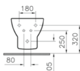
Without side holes
