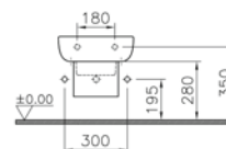
Standard connection
