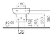
Concealed connection
