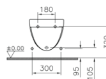
With side holes
