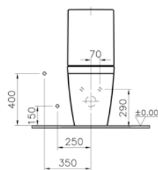
Concealed water connection
