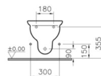
With side holes
