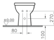
Without side holes
