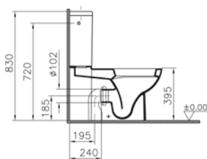
Side inlet
