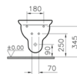
Without side holes
