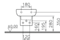
Concealed connection
