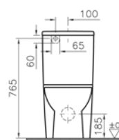
Back inlet
