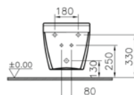
Without side holes
