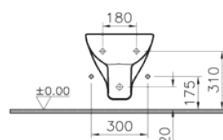
Without side holes
