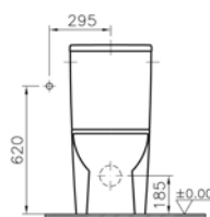
Side inlet
