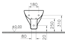
With side holes
