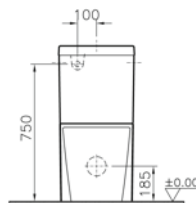
Back inlet
