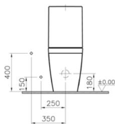
Water connection from side
