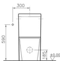
Side inlet
